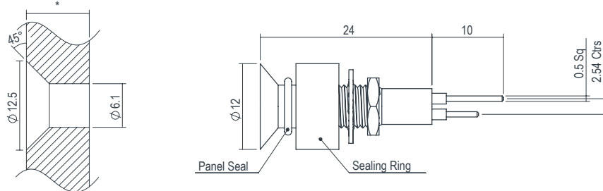
Panel and Mounting Hole
